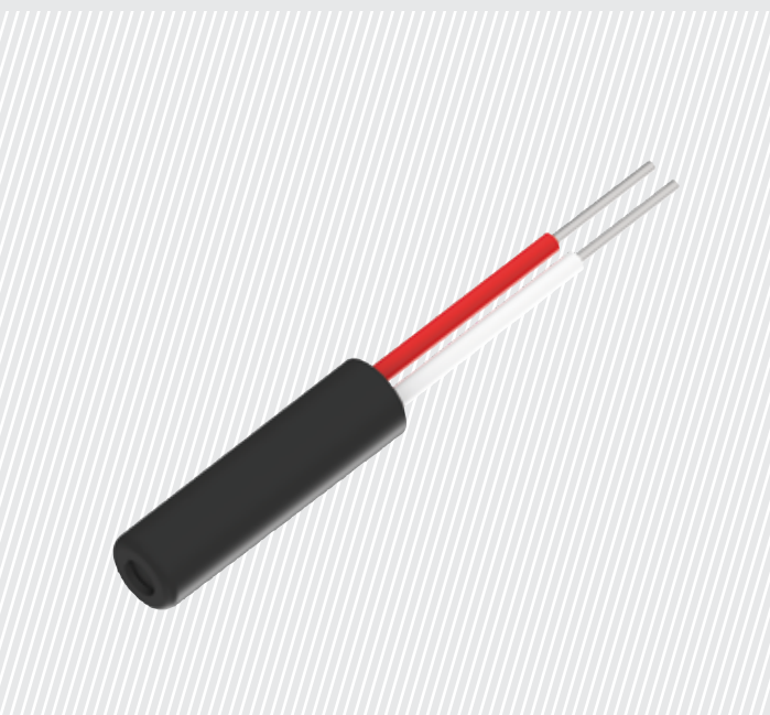
PT1000 temperature sensor integrated in the charging connection or in the electric drive motor
